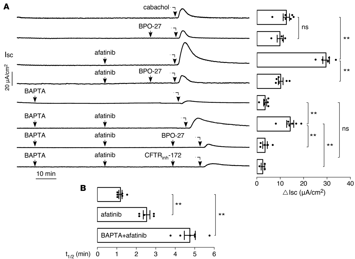
Figure 3. The afatinib-induced augmentation in carbachol current is CFTR dependent. (A) (Left) short-circuit current in T84 cells showing effects of 20 \mu\text{M} afatinib, 100 \mu\text{M} carbachol, 10 \mu\text{M} BPO-27, and 10 \mu\text{M} CFTR inh -172, with or without 30 \mu\text{M} BAPTA-AM, as indicated. (Right) summary of peak carbachol-induced current (mean \pm SEM, n = 3-6 ). (B) Half-time ( t_{1/2} ) of the decreasing phase of the carbachol response curve (mean \pm SEM, n = 5-6 ). ** P < 0.01 , by 2-tailed t test.
